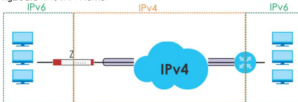
Figure 272 IPv6-in-IPv4 Tunnel
