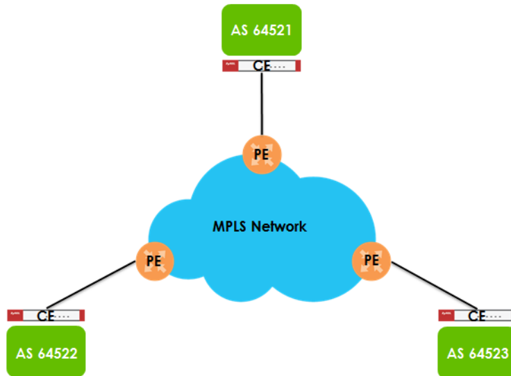
Figure 312 Scenario 1: CE Router – to – MPLS
