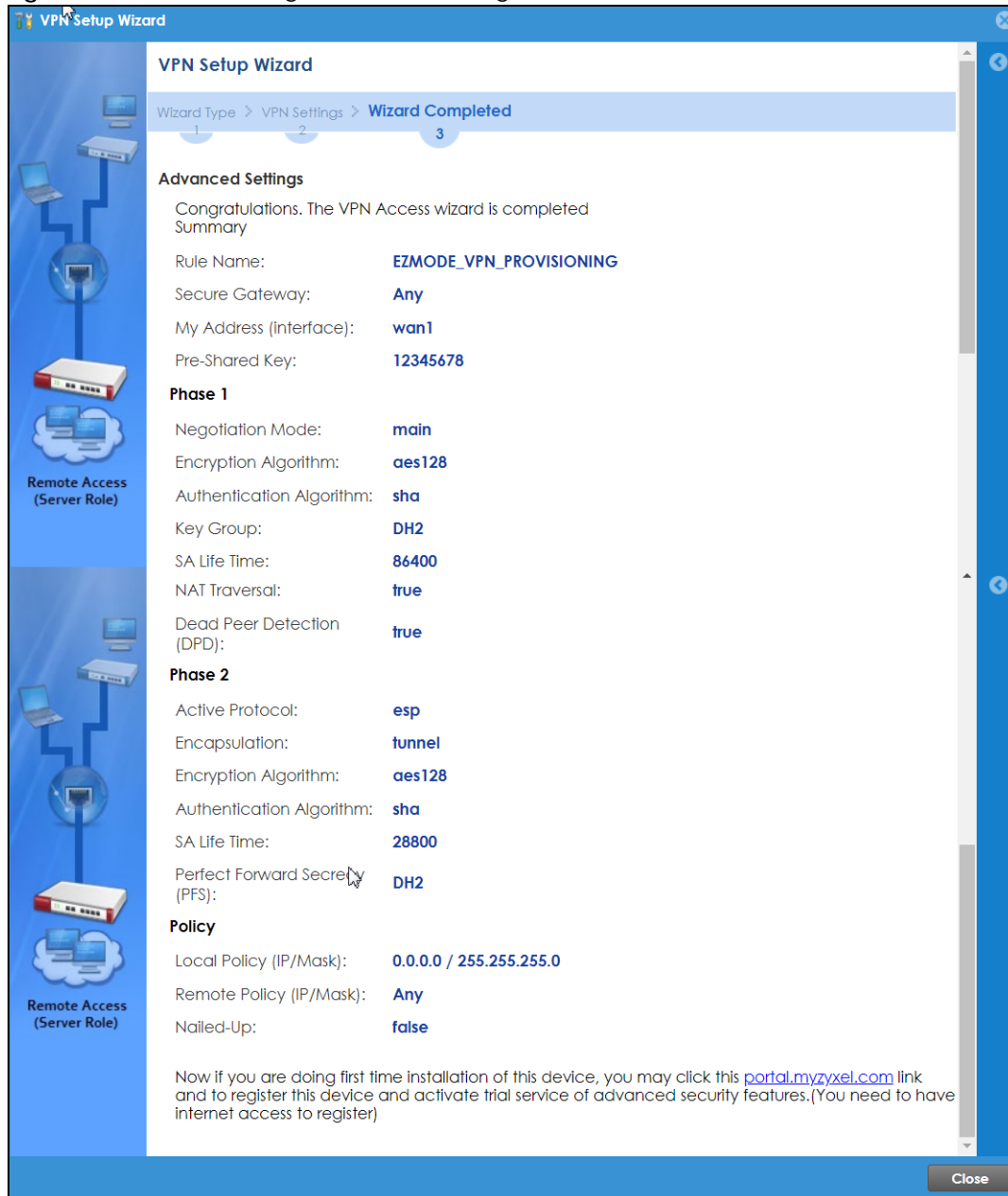
Figure 104 VPN for Configuration Provisioning Advanced Wizard: Finish
