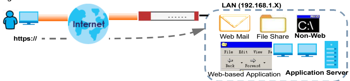
Figure 439 SSL VPN
