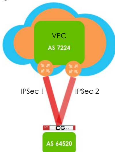
Figure 436 CG – to – Amazon VPC
