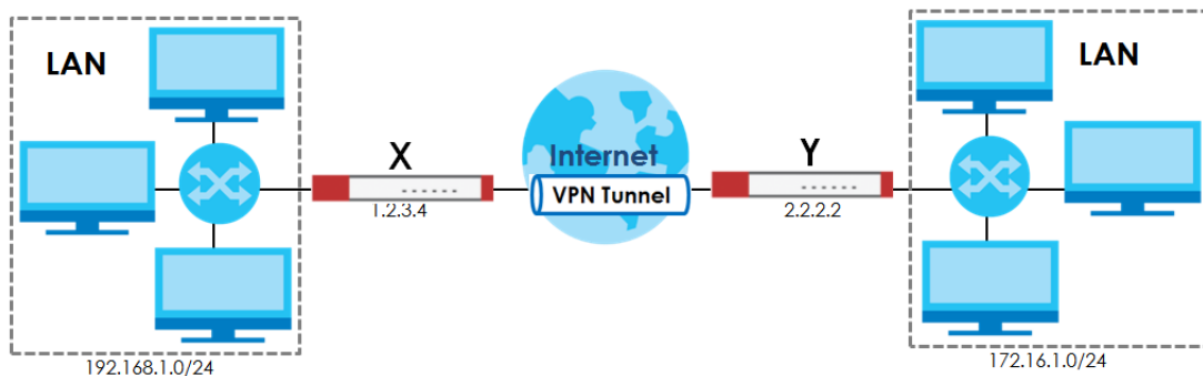
Figure 456 Site-to-site IPsec VPN Example
