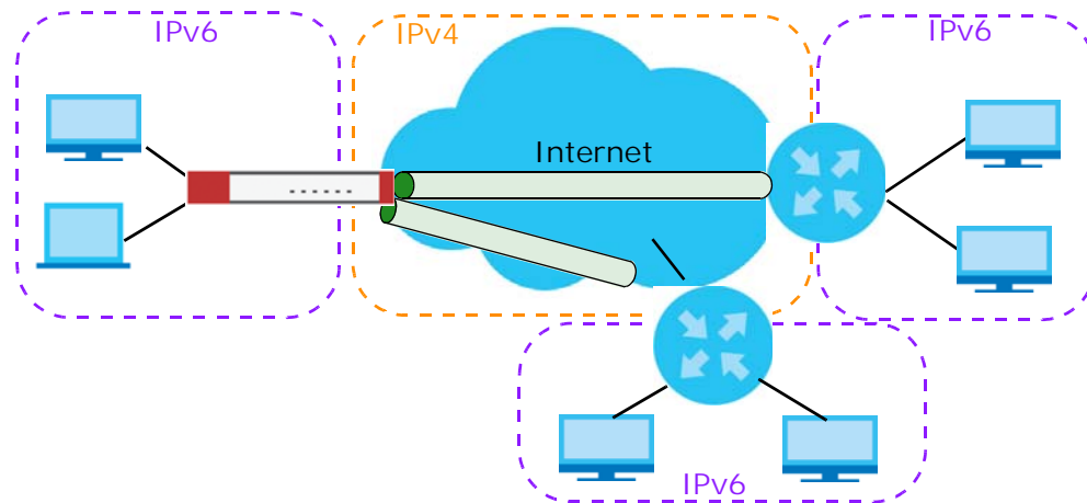
Figure 273 6to4 Tunnel
