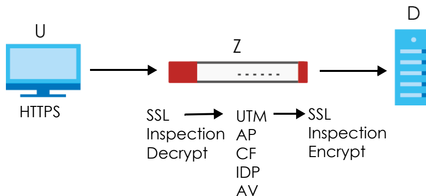
Figure 536 SSL Inspection Overview
