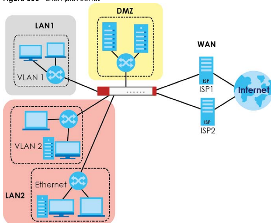
Figure 553 Example: Zones
