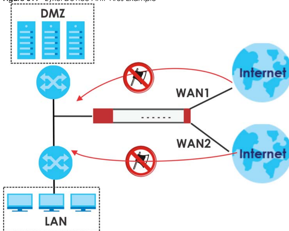
Figure 519 Zyxel Device Anti-Virus Example
