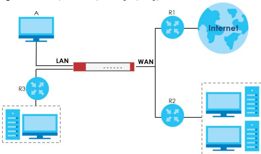
Figure 294 Example of Policy Routing Topology
